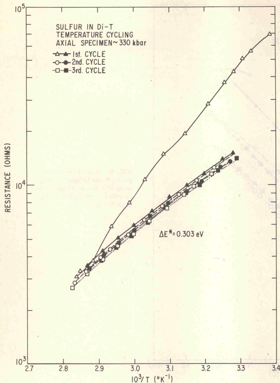
FIG. 4. \log R vs 10^3/T(^{\circ}\text{K}) plot for temperature-cycling of axial specimen of sulfur 330 kbar pressure.
